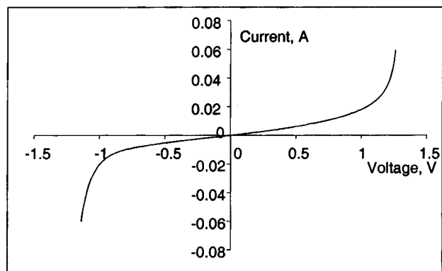
FIG. 3. Typical I – V curve for an Al/ a -CdTe:O/Pb tunnel junction. The slope change from 0 V to approximately ±0.6 V is typically 10%–30% and is asymmetric with bias polarity.
